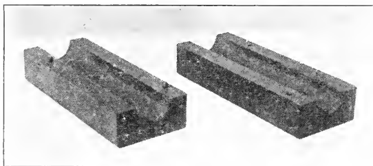
FIG. 537. TWO-PART CORE-BOX.
